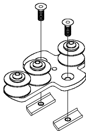
top cord cord guide pulley 18-85-13
