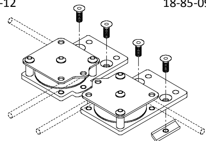
top cord side entry pulley 18-85-
