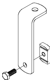
top cord hanger bracket 18-85-31
