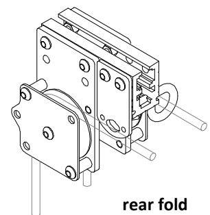
rear fold return pulley 18-00-07-RF
