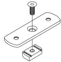
soffit mounting clip 18-00-29
