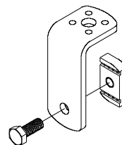
stand-off bracket 18-85-42
