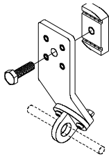
line guide 18-85-40
