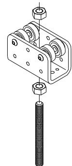
heavy duty scenery carrier 18-00-37
