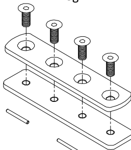
joint set 18-85-24
