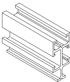
6m std length 18-8541-6
