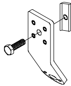
end stop-eye 18-85-41
