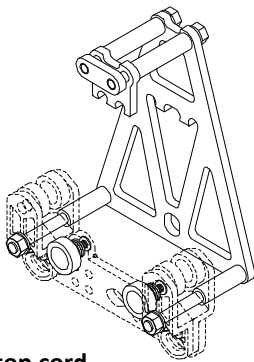
top cord master carrier bracket 18-85-04
