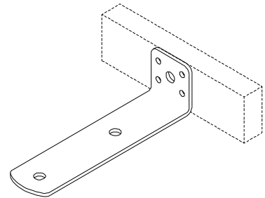
valance bracket 160/80mm 18-00-43
