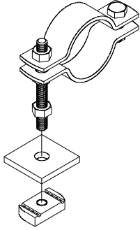
batten clip & threaded rod hanger assemblies
