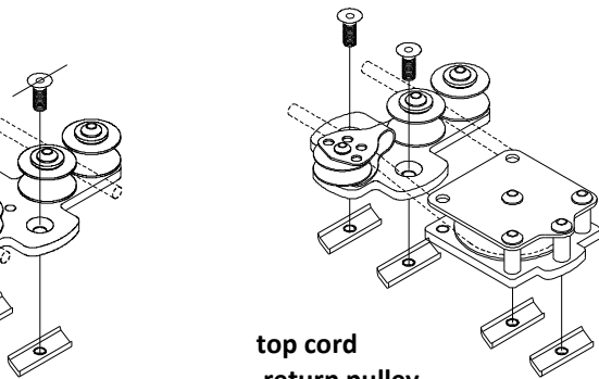
top cord return pulley 18-85-09
