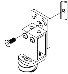
outrigger pulley 18-85-22
