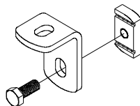
soffit mount hanger bracket 18-85-35
