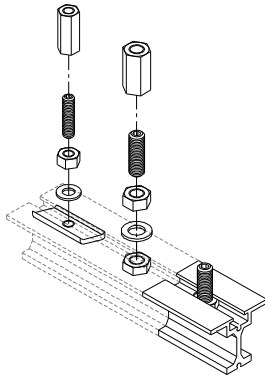
threaded rod / socket hanger assemblies
