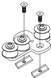
top cord master carrier bracket 18-85-04
