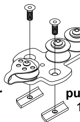
top cord return pulley feeder 18-00-12
