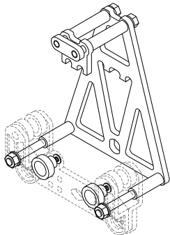
top cord master carrier bracket 18-85-04
