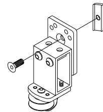
outrigger pulley 18-00-21-B
