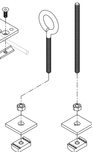
eyebolt assembly
